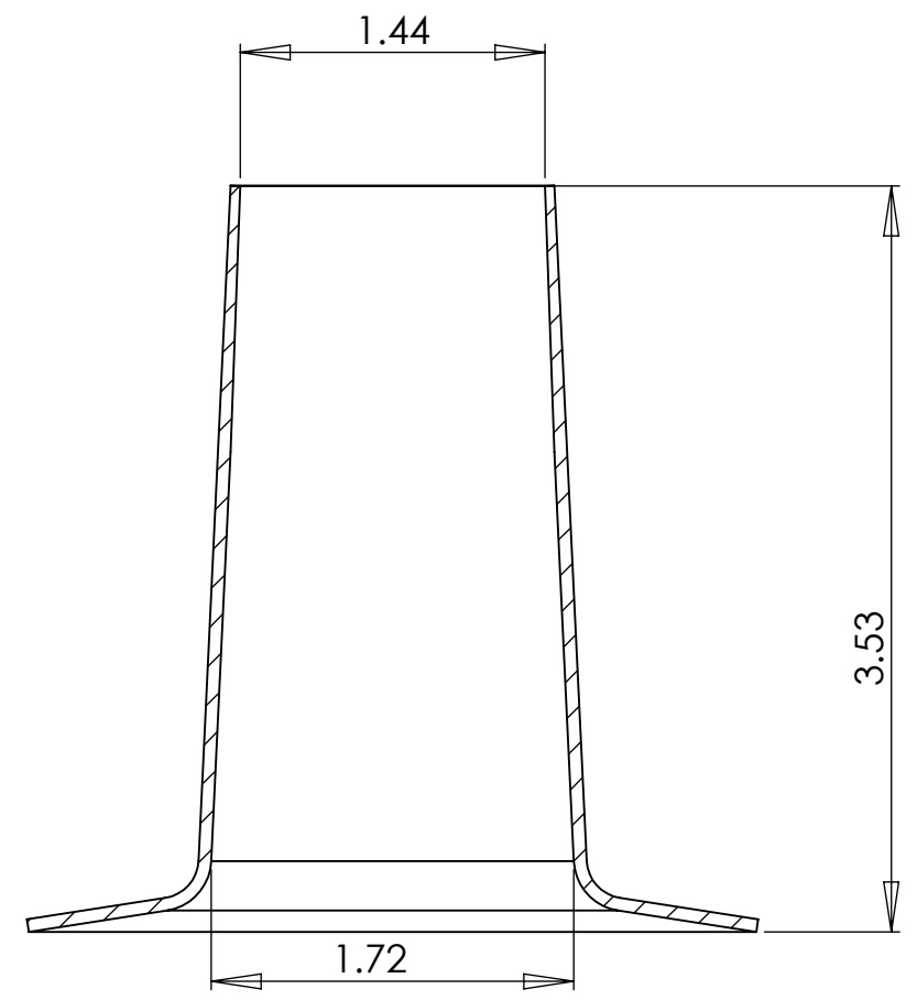
SECTION C-C SCALE 1 : 1
